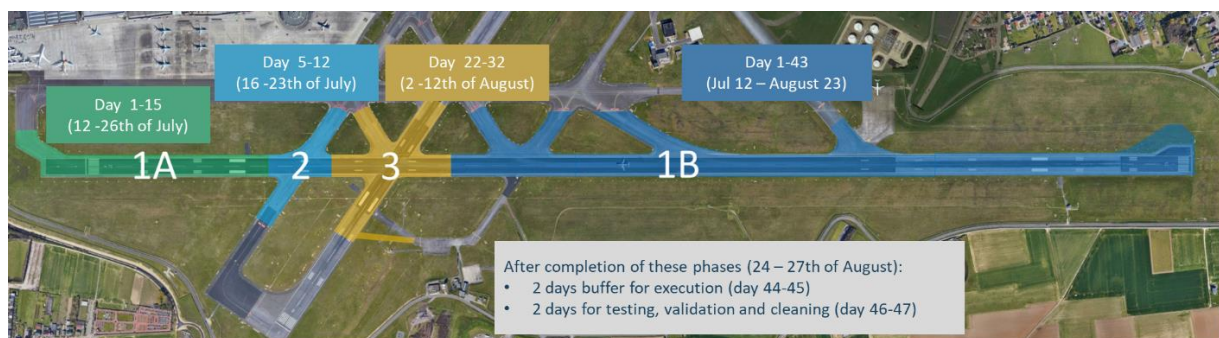
Figure 1: Detail of phases and timing of RWY 25L renovation works
